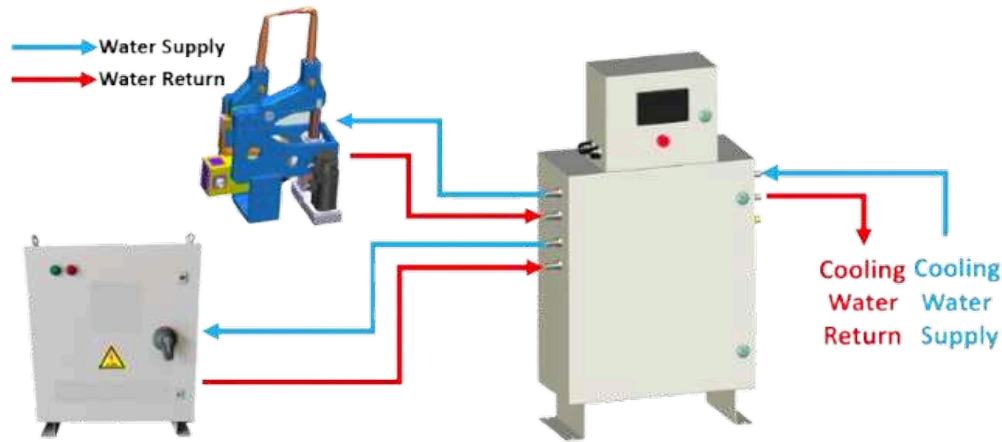
Water Connection Diagram
